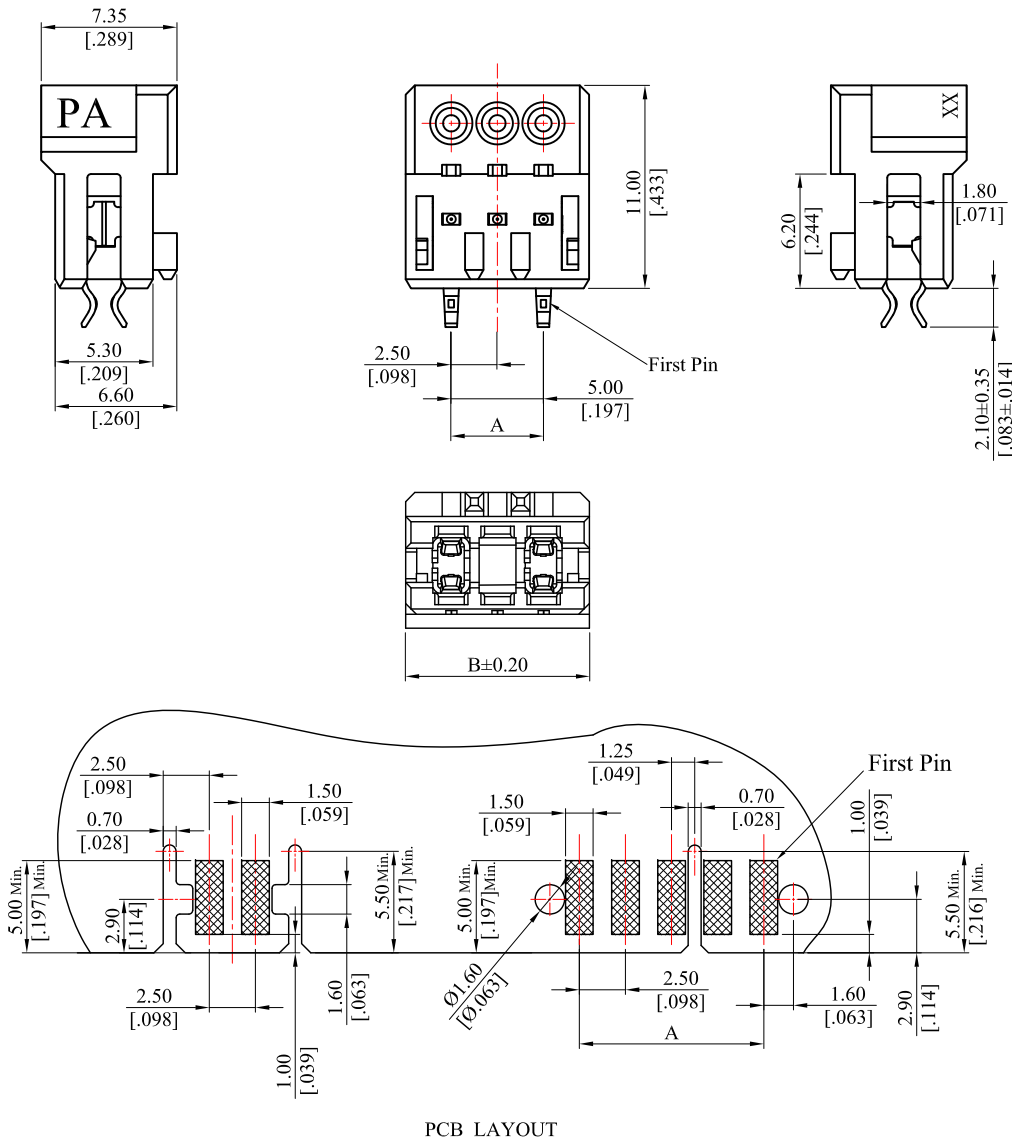
PCB LAYOUT
